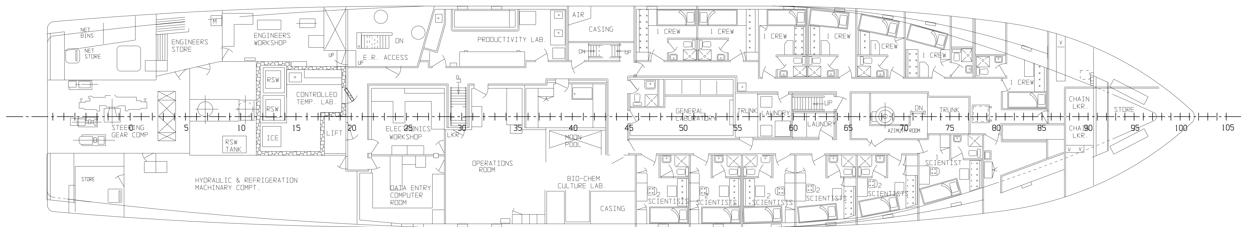
MAIN DECK
