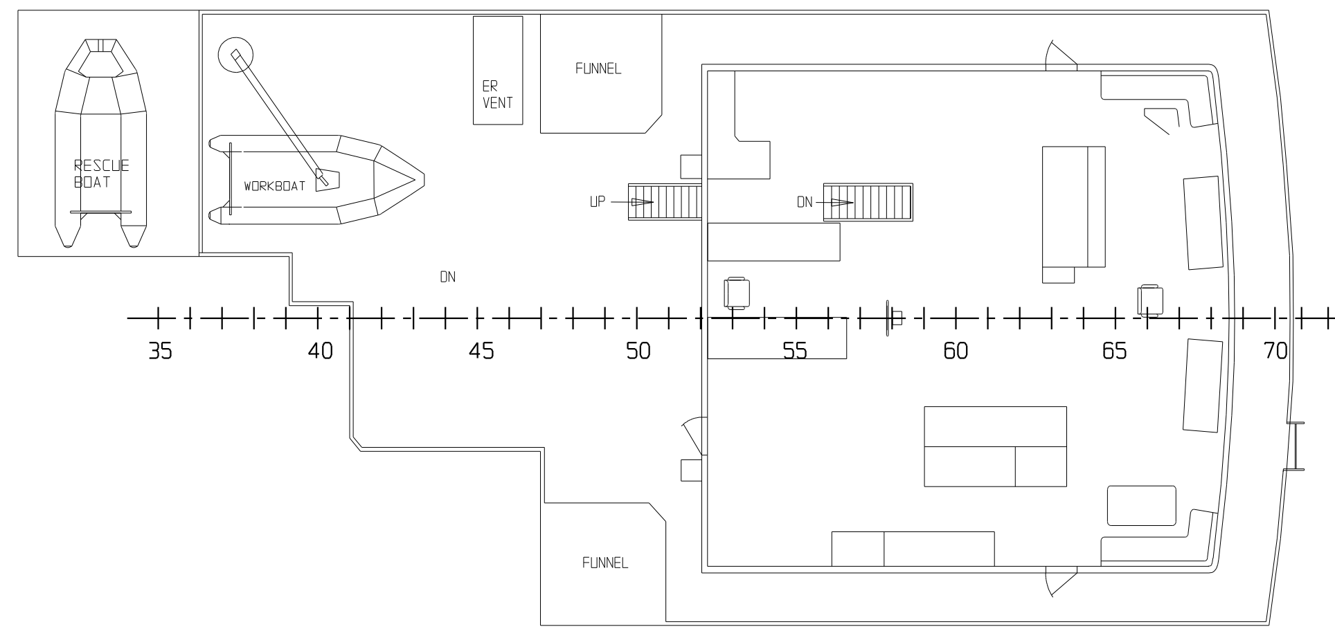
BRIDGE DECK
