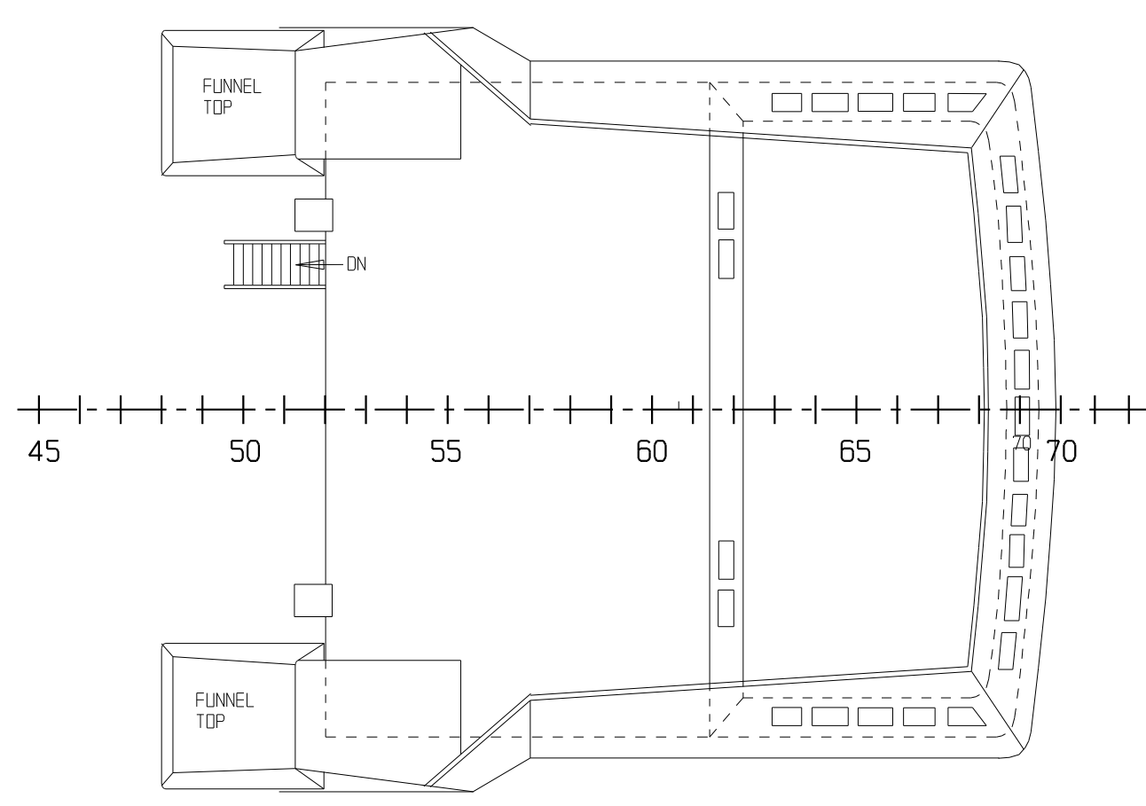
WHEELHOUSE ROOF
